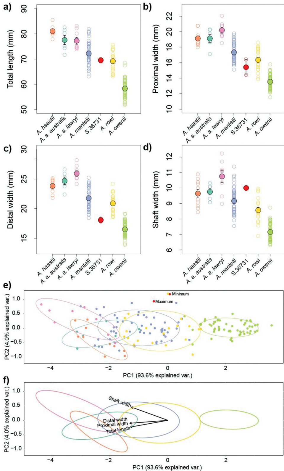
Figure 2. Plots showing the measurements of the kiwi taxa analysed. (a) tarsometatarsus length; (b) proximal width; (c) distal width; (d) shaft width; (e) biplot with scores of the principal components 1 and 2 showing the clustering of the different taxa relative to the Marton fossil (using either the minimum or maximum estimated values); (f) projection of the principal component vectors (loadings) onto the PC1-PC2 biplot showing the direction of the measurement vectors. Colours represent different taxa. Filled circles represent a mean (Figs a–d) or a single value (Fig. e), while open circles (Figs a–d) represent the individual measurements used to calculate the mean. For the Marton kiwi, the mean and individual points are based on the minimum and maximum possible value for each measurement. Error bars (Figs a–d) indicate standard errors. Ellipses (Figs e and f) are normal data ellipses (68% probability for each group).
