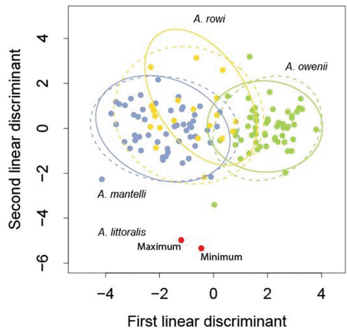
Figure 3. Biplot showing the results of the linear discriminant analysis for A. mantelli (blue), A. rowi (yellow), A. owenii (green) and the Marton fossil (red) and the distance of the Marton fossil to the centre of the ellipses as described in Table 2. With the exception of the Marton fossil, each point represents a single specimen and ellipses are 95% confidence ellipses for each group. Dashed ellipses represent our original classification while solid line ellipses represent the model classification.
